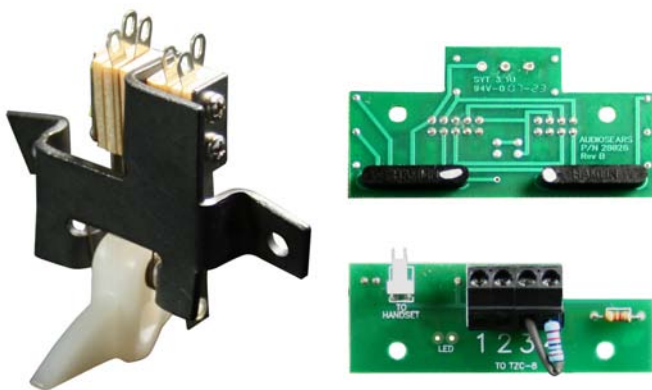
Switches - mechanical leaf or magnetic reed switch
